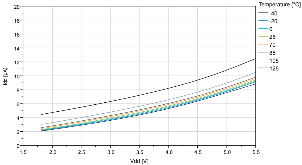
Figure 35-9. Idle Supply Current vs. V_{DD} ( f=32\text{KHz OSC} \text{ULP32K} )
