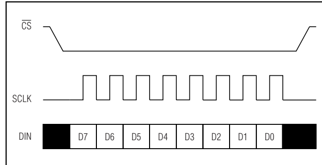
Figure 6. 3-Wire Serial-Interface Operation for the MAX4823
