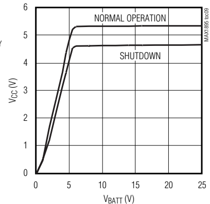
V_{CC} vs. V_{BATT}
