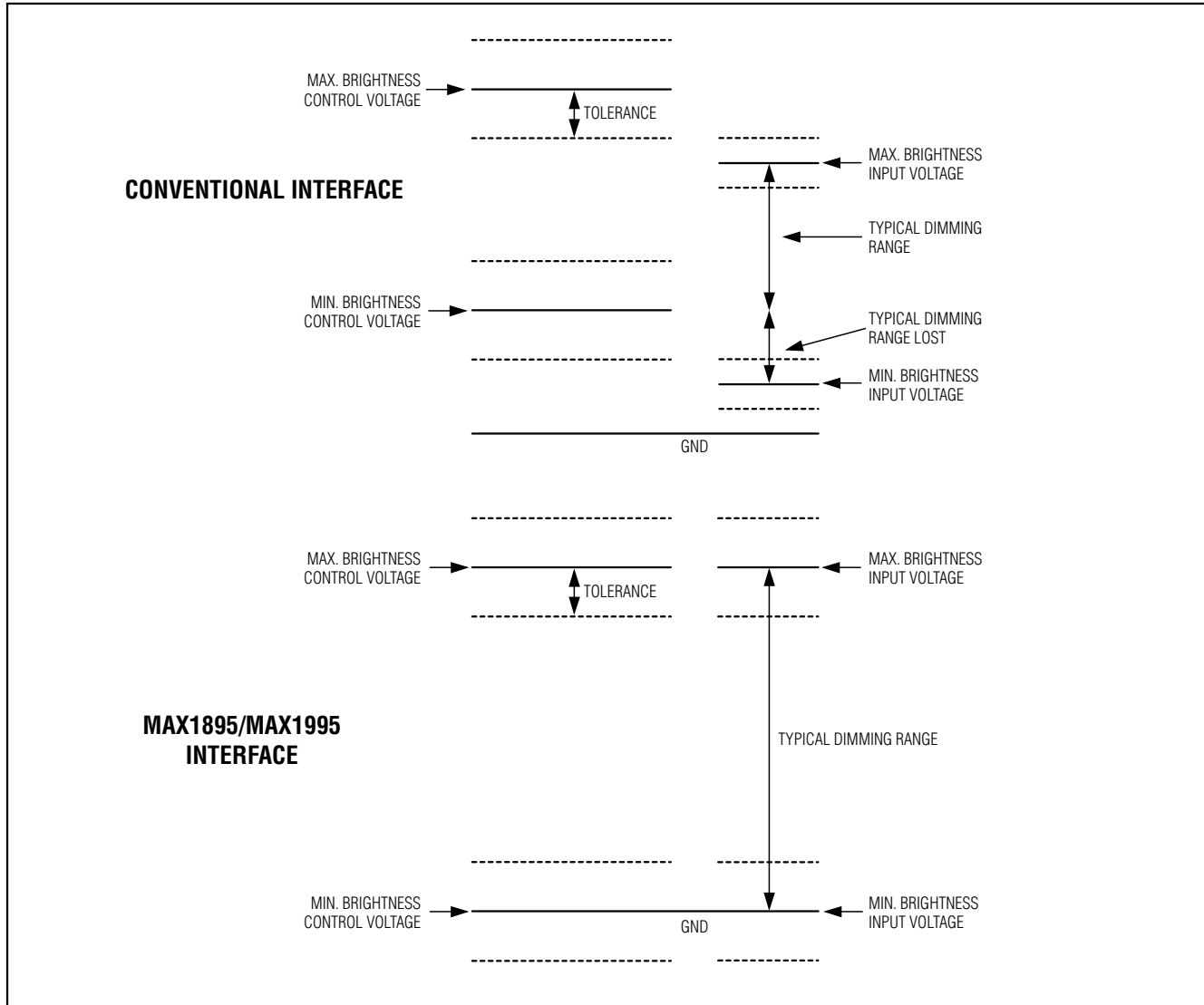
Figure 9. Useful Dimming Range
