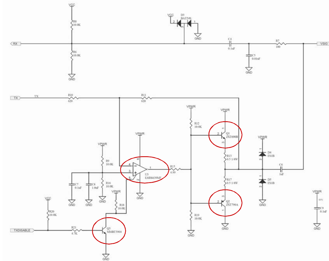
Figure 3-9. Transmit Filter, Transmit Amplifier, and Receive Filter
