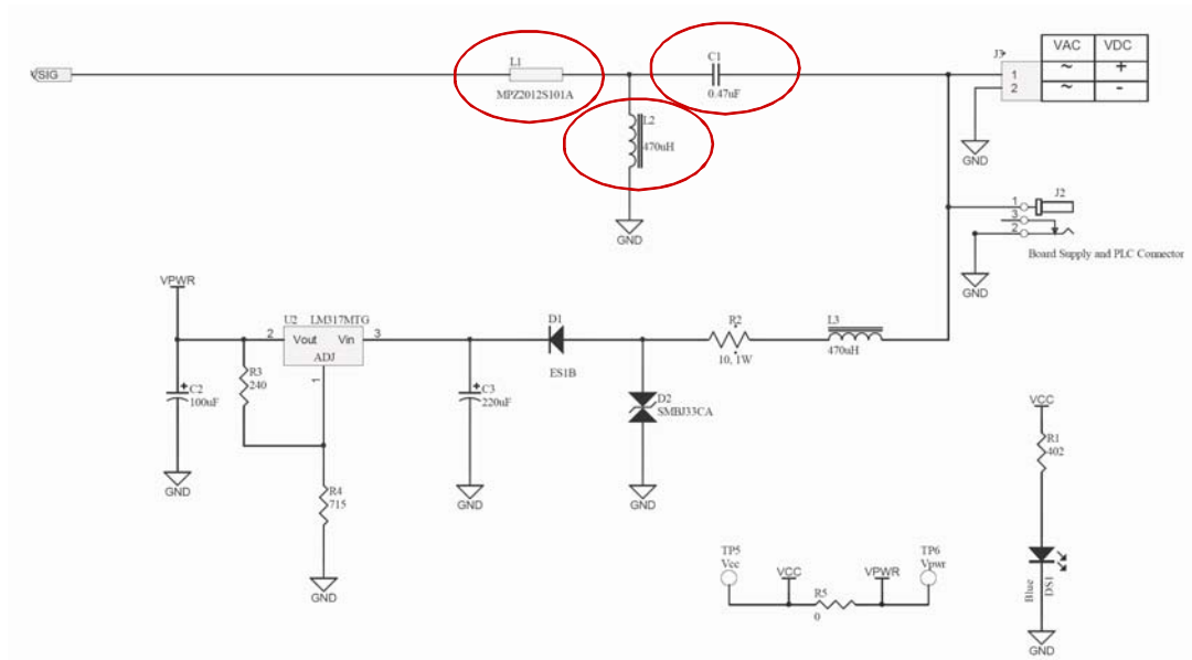
Figure 3-10. Coupling Circuit
