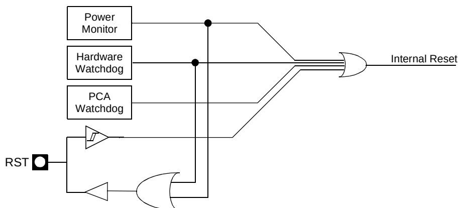
Figure 16. Reset Schematic
