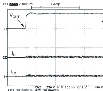
Figure 16. Start-Up at V_{IN} = 265 V_{RMS} , P_{OUT} = 0 W
