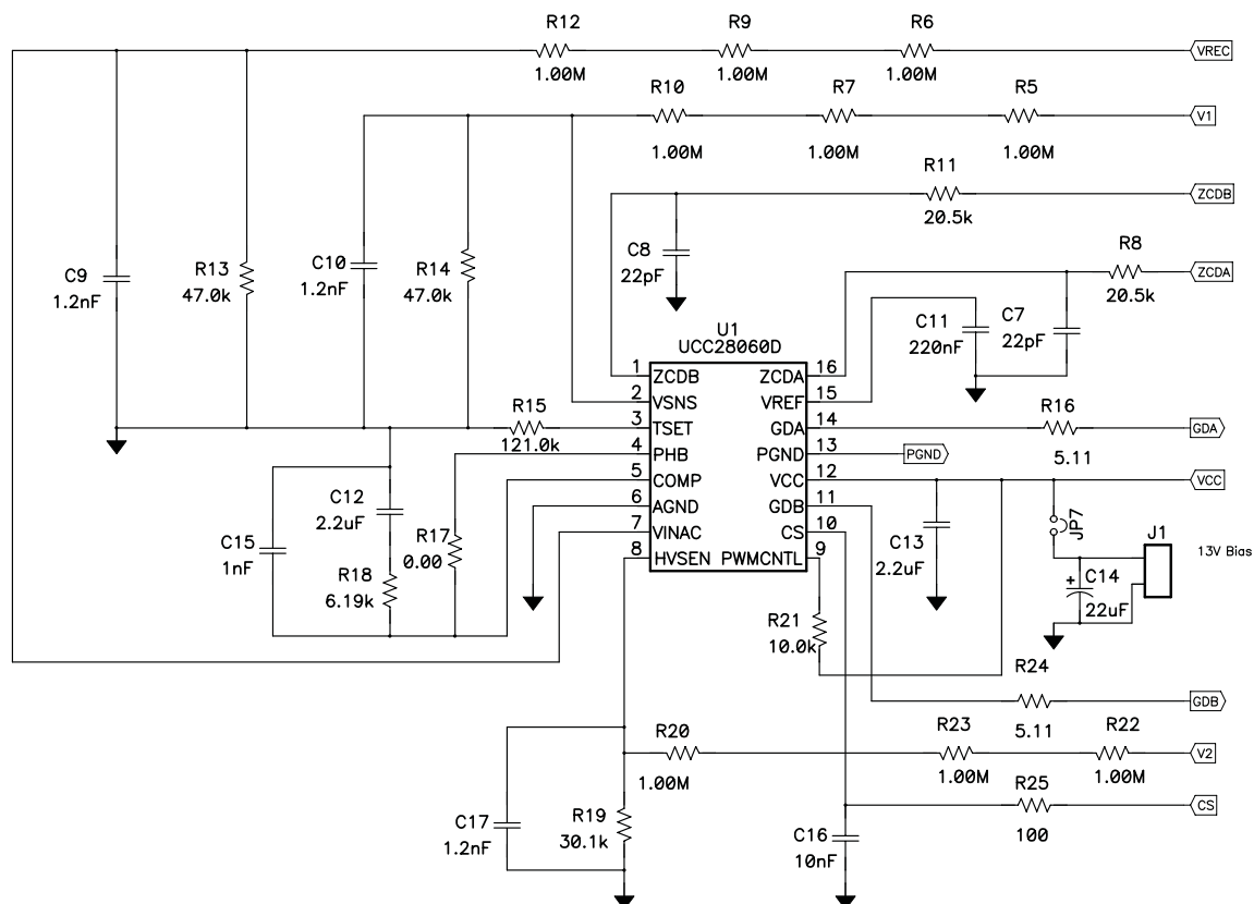
Figure 2. Controller Circuitry
