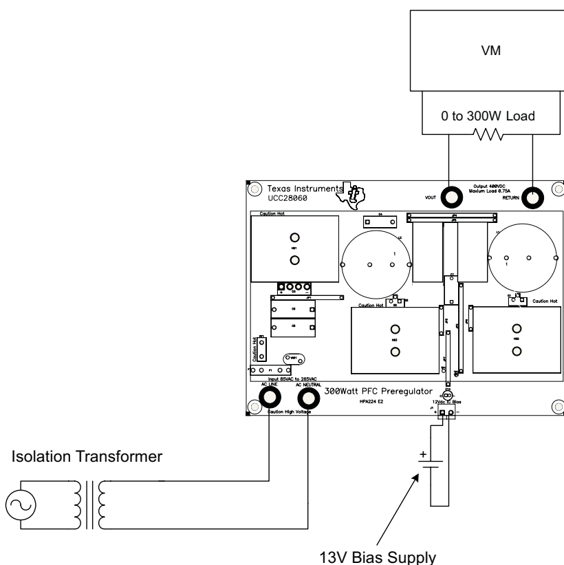
Figure 3. Test Setup
