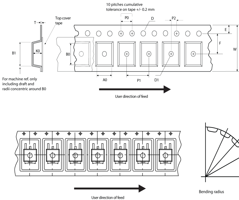
Figure 47. Tape outline
