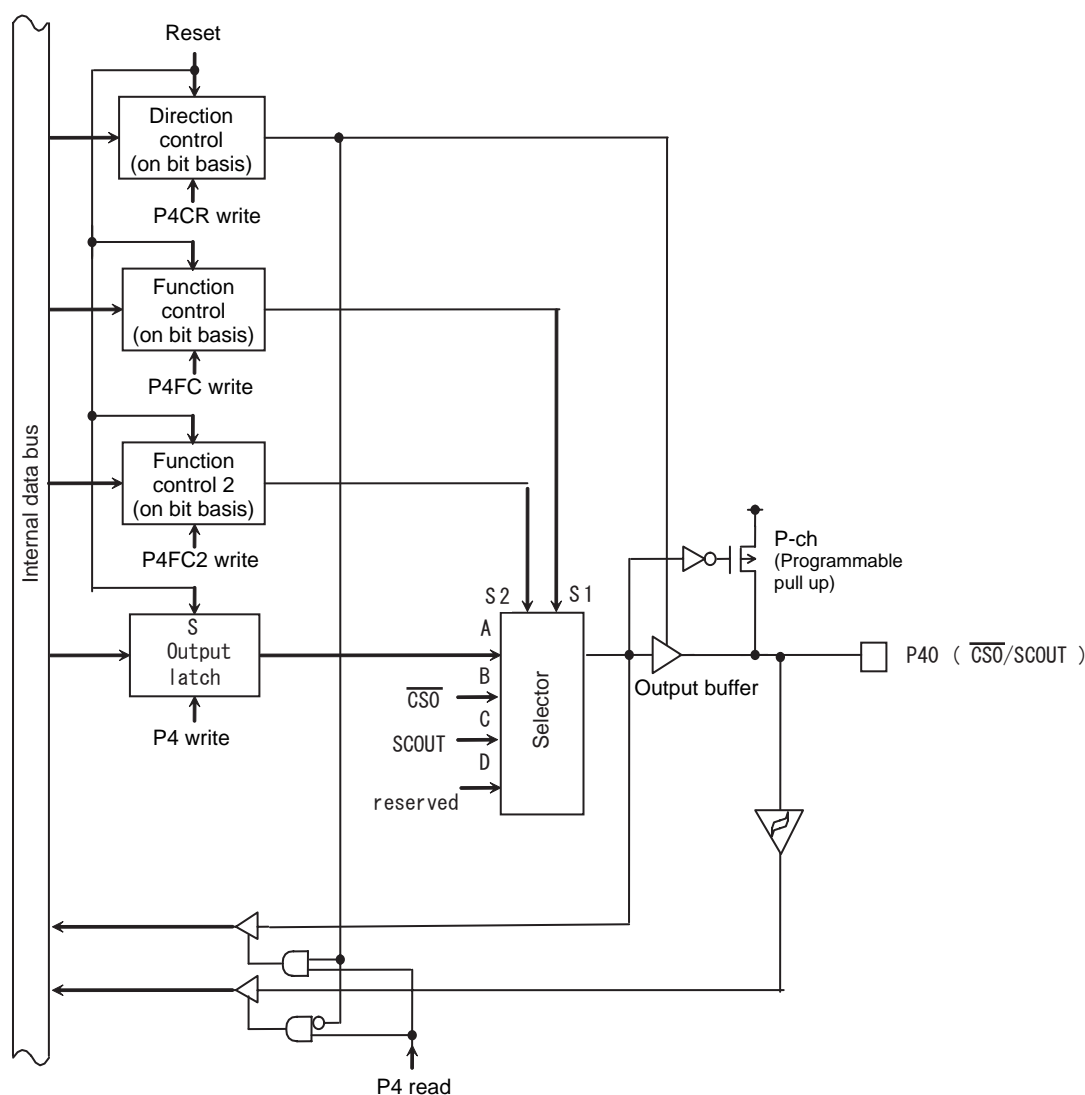
Figure 4-6 Port 40
