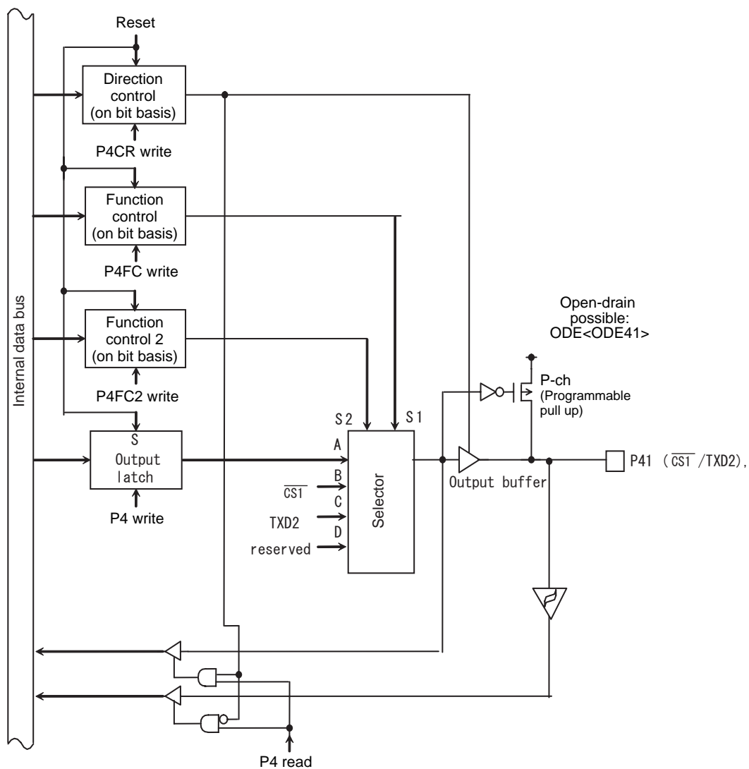
Figure 4-7 Port 41
