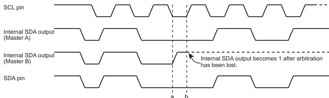
Figure 9-7 Arbitration Lost
