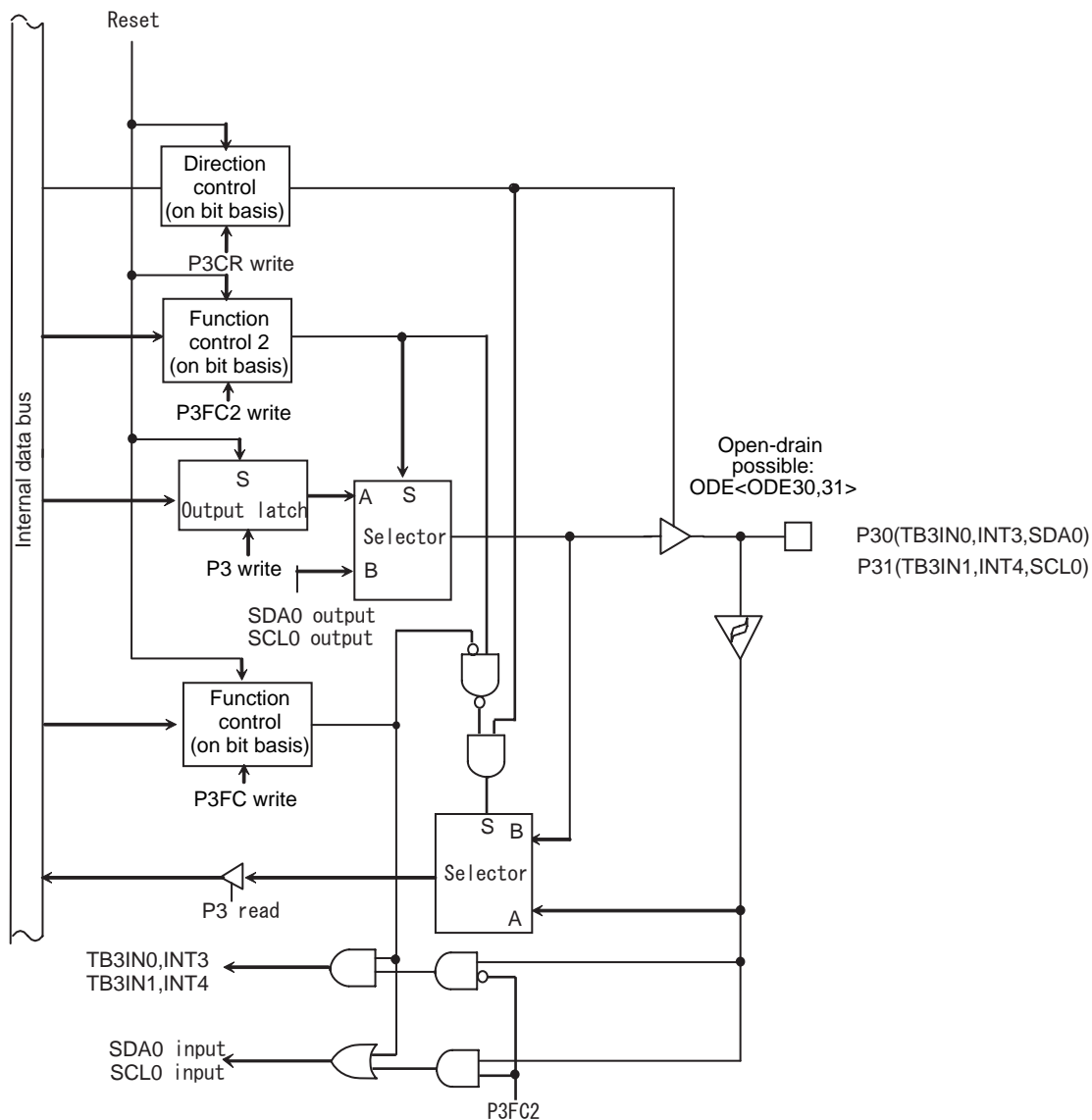
Figure 4-4 Port 30 and 31
