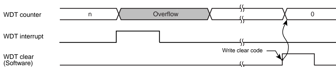
Figure 12-2 Normal Mode
