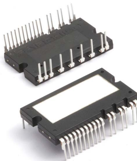
Figure 1. Package Overview
