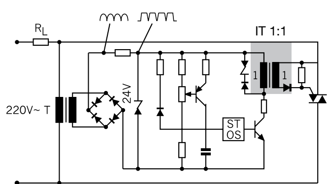
Triac phase angle control
