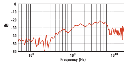
Figure 3.5. Common mode rejection vs. frequency.
