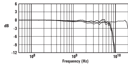
Figure 3.4. Swept frequency response.
