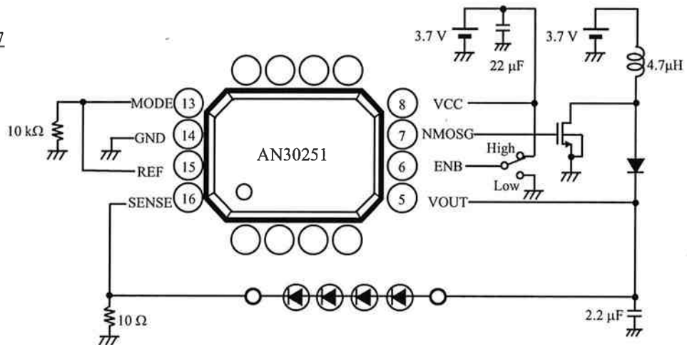
Test Circuit 7
