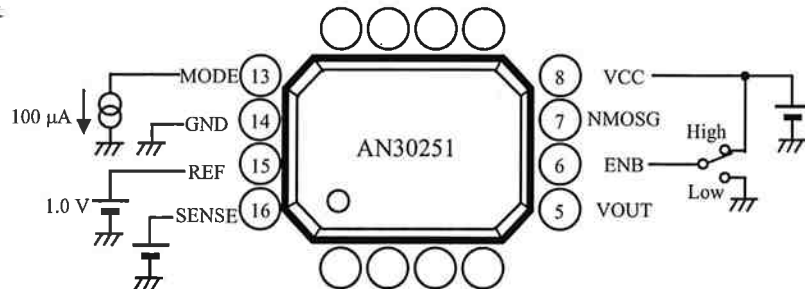
Test Circuit 5
