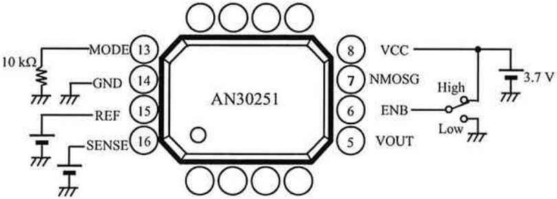
Test Circuit 3
