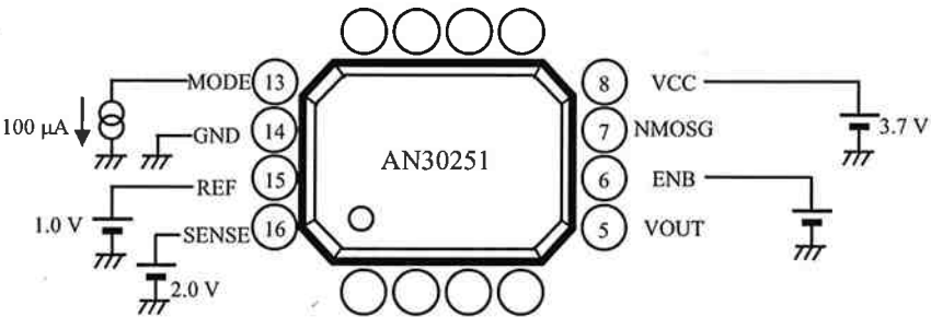
Test Circuit 2
