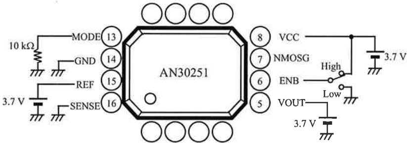
Test Circuit 1
