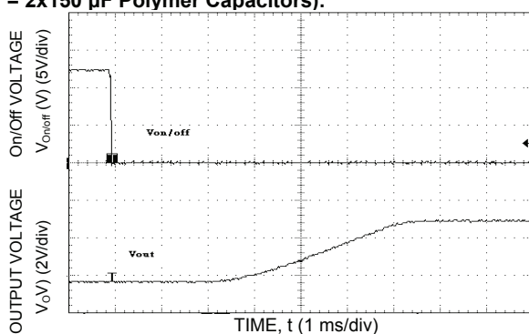
Figure 14. Typical Start-Up Using Remote On/Off ( V_{in} = 12 Vdc, V_o = 3.3 Vdc, I_o = 5.0 A).
