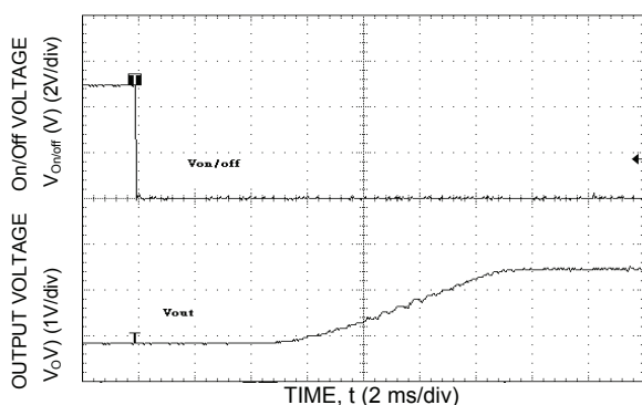
Figure 15. Typical Start-Up Using Remote On/Off with Low-ESR external capacitors (7x150uF Polymer) ( V_{in} = 12 Vdc, V_o = 3.3 Vdc, I_o = 5.0 A, C_o = 1050 \mu F).
