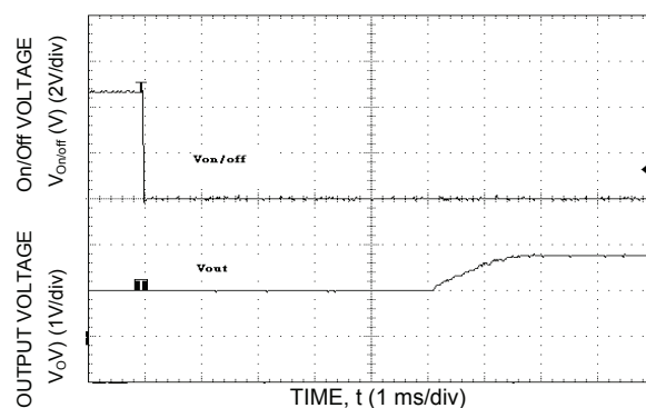
Figure 17 Typical Start-Up using Remote On/off with Prebias ( V_{in} = 12 Vdc, V_o = 1.8 Vdc, I_o = 1 A, V_{bias} = 1.0 Vdc).
