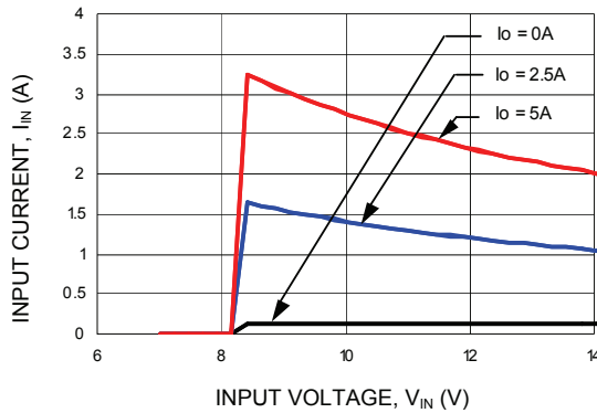
Figure 7. Input voltage vs. Input Current ( V_{out} = 5.0\text{Vdc} ).
