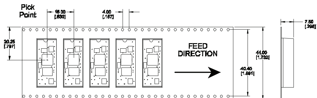
Surface Mount Tape & Reel
