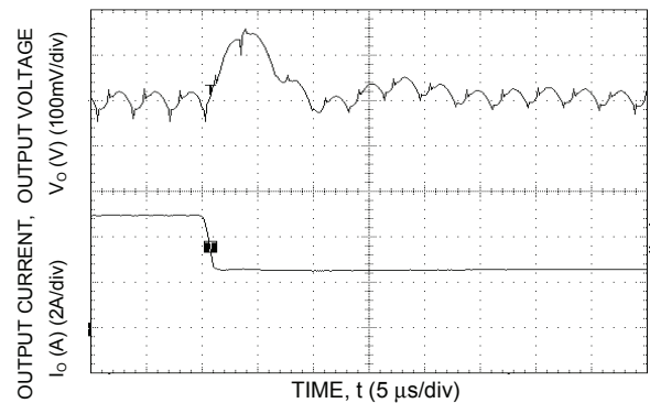
Figure 11. Transient Response to Dynamic Load Change from 100% to 50% of full load ( V_o = 3.3\text{Vdc} ).
