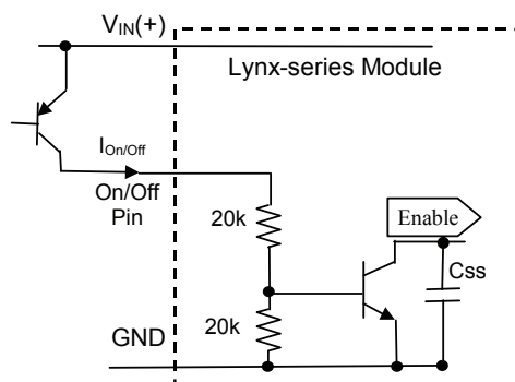
Figure 27. Remote On/Off Implementation
