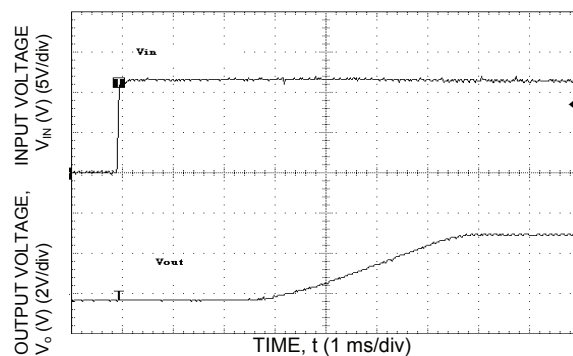
Figure 16. Typical Start-Up with application of V_{in} with ( V_{in} = 12 Vdc, V_o = 3.3 Vdc, I_o = 5 A).
