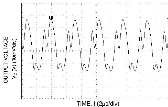
Figure 9. Typical Output Ripple and Noise ( V_{in} = 12.0\text{V dc} , V_o = 5.0\text{Vdc} , I_o = 5\text{A} ).
