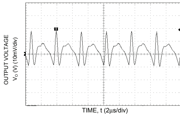
Figure 8. Typical Output Ripple and Noise ( V_{in} = 12\text{V dc} , V_o = 0.75\text{Vdc} , I_o = 5\text{A} ).
