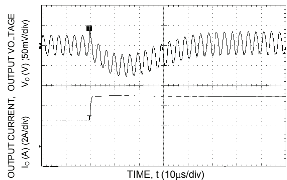
Figure 12. Transient Response to Dynamic Load Change from 50% to 100% of full load ( V_o = 5.0\text{Vdc} , C_{ext} = 2 \times 150\text{ }\mu\text{F} Polymer Capacitors).
