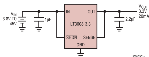
3.3V, 20mA Supply with Shutdown
