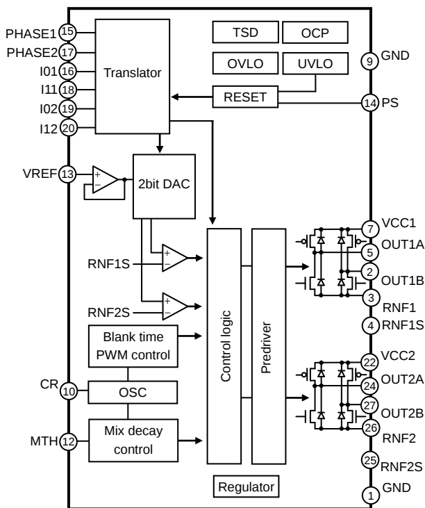
Figure.3 Block Diagram
