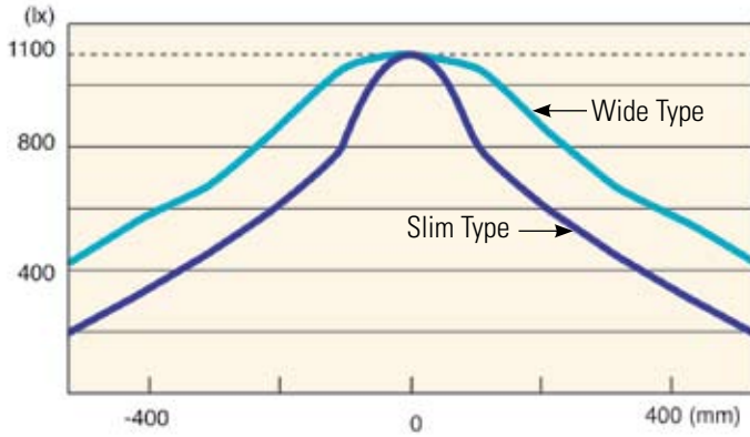
Light Distribution at 1.0m LF1D
