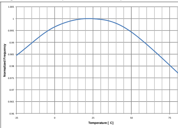
Figure 5. Frequencies vs temperature
