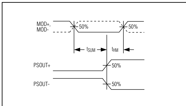
Figure 1. Timing Diagram
