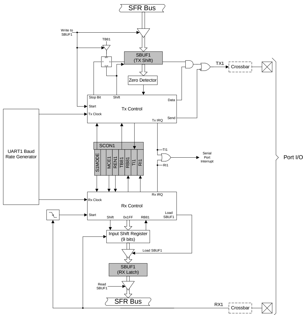
Figure 23.1. UART1 Block Diagram
