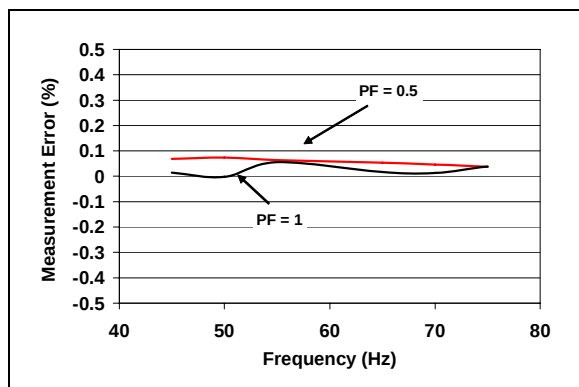
FIGURE 2-15: Measurement Error vs. Input Frequency.
