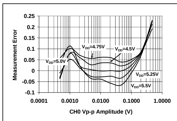
FIGURE 2-20: Measurement Error vs. V_{DD} , G = 16 , External V_{REF} .
