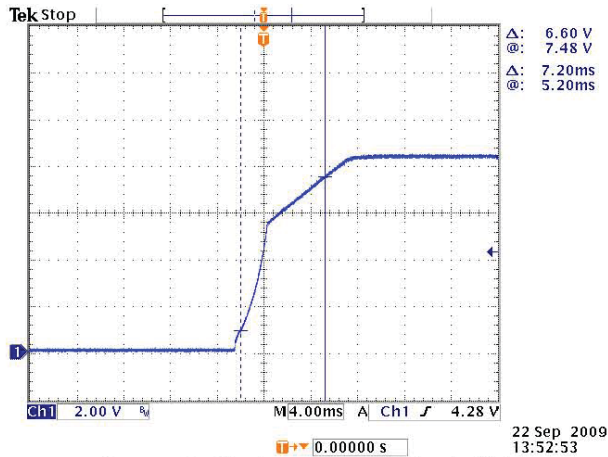
Step Load Transient Response ( V_{in} = 48V , Resistive load, C_{out}=0 , I_{out}=75\% to 50% of I_{max} , T_a=+25^{\circ}C .)
