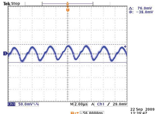
Output Ripple and Noise ( V_{in} = 48V , I_{out}=0A , C_{load}=1\mu F ceramic II 10\mu F tantalum, T_a=+25^{\circ}C , ScopeBW=20MHz)
