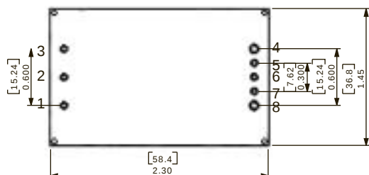
OPEN FRAME (NO BASEPLATE) PIN SIDE VIEW
