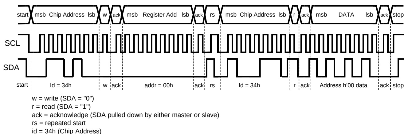
Figure 21. Read Cycle
