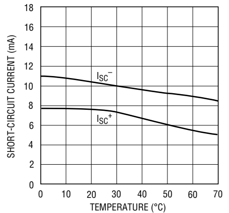
Driver Short-Circuit Current vs Temperature
