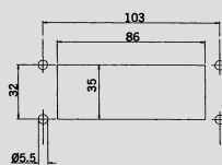
Cut-out size 16 35 x 86 mm
