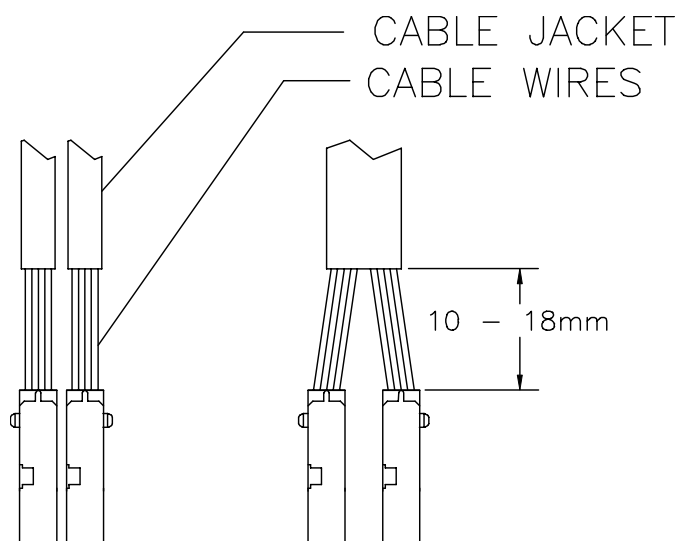
Figure 7 Dimensions - Single Or Multiple Cables per Unshielded Connector
