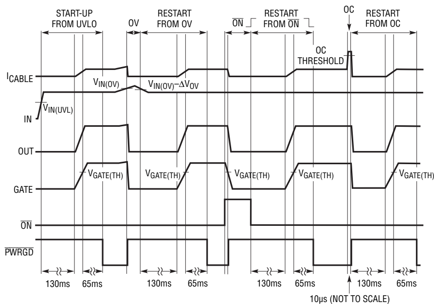
Figure 2. \overline{PWRGD} Behavior
