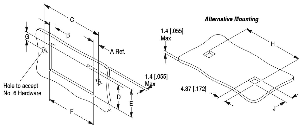
6.35 [.250] Series Panel Cutout
