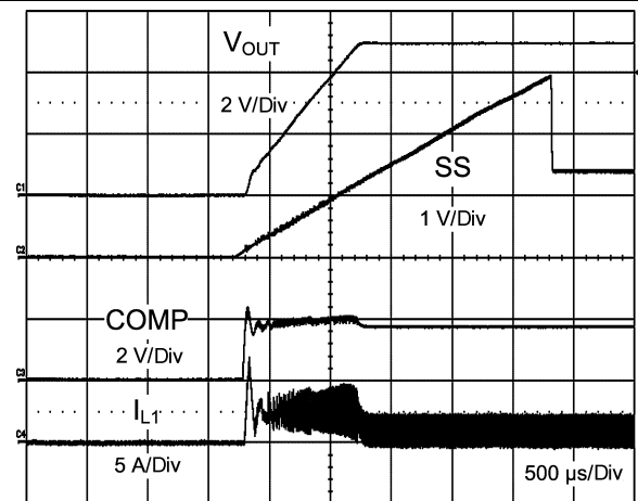
Figure 41. Short Circuit Recovery Into Resistive Load With C7 = 1 μF and D2 Installed
