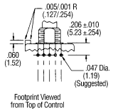
Footprint Viewed from Top of Control
