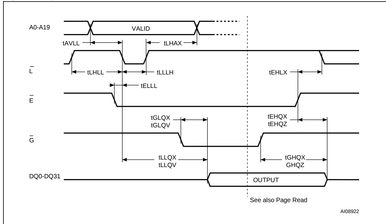
Figure 9. Asynchronous Latch Controlled Bus Read AC Waveforms
