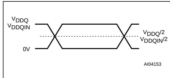
Figure 6. AC Measurement Input Output Waveform
