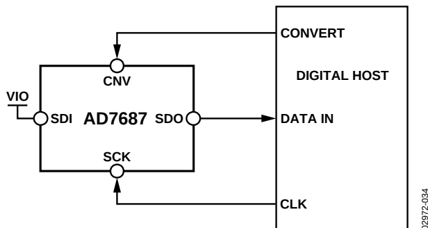
Figure 35. \overline{\text{CS}} Mode 3-Wire, No BUSY Indicator Connection Diagram (SDI High)
