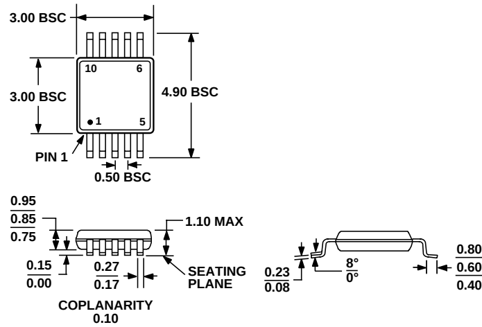
Figure 49. 10-Lead Mini Small Outline Package [MSOP] (RM-10)
