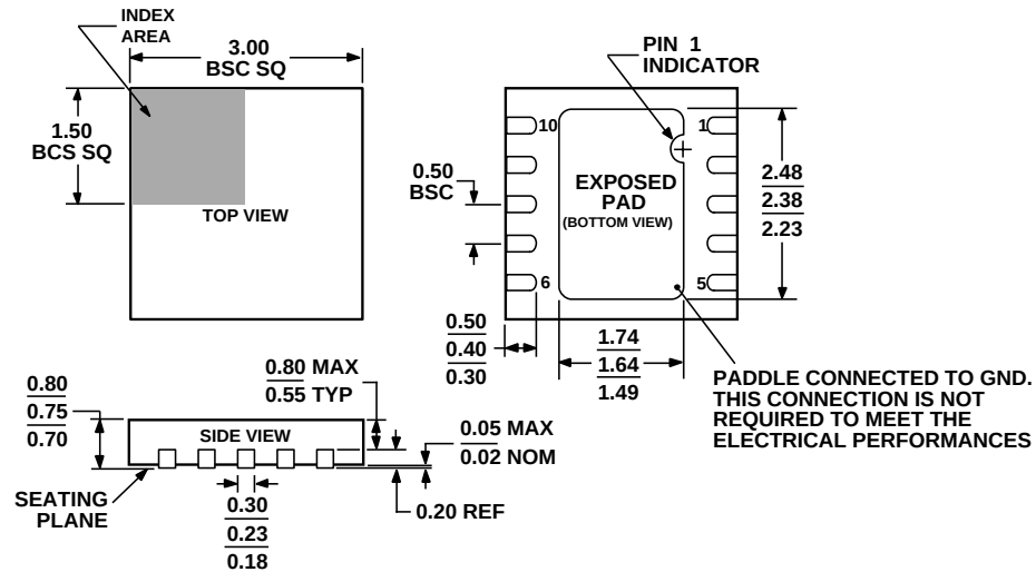
Figure 50. 10-Lead Lead Frame Chip Scale Package [QFN 1 (LFCSP_WD)] 3 mm × 3 mm Body, Very Very Thin, Dual Lead (CP-10-9)
