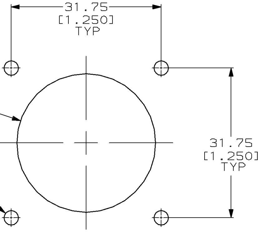
FRONT MOUNTED PANEL CUTOUT
