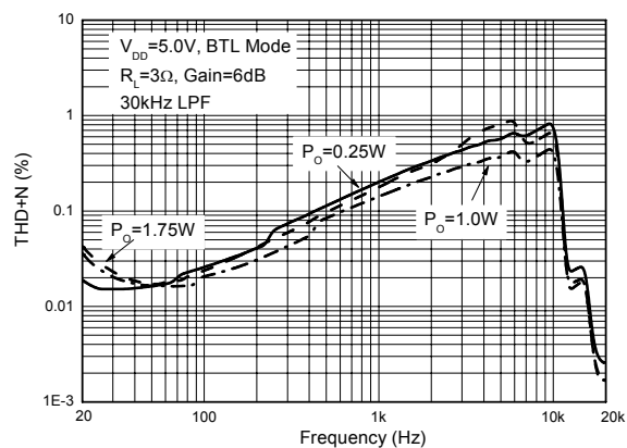
Figure 16. THD+N vs. Frequency
