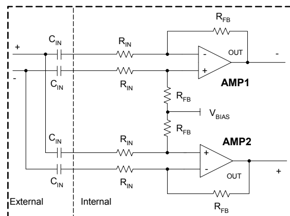
B) Classic Input Configuration with Input Capacitor
