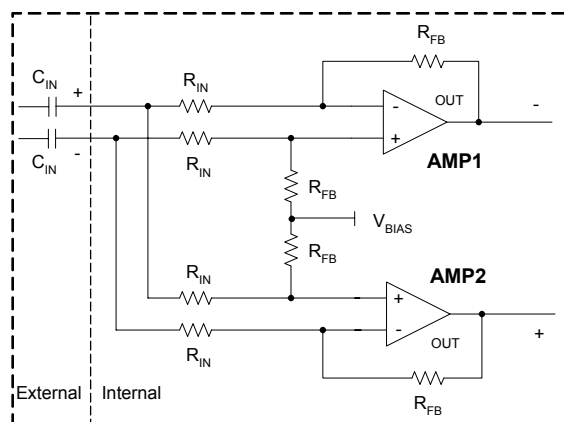
A) AA4006 Input Configuration with Input Capacitor
