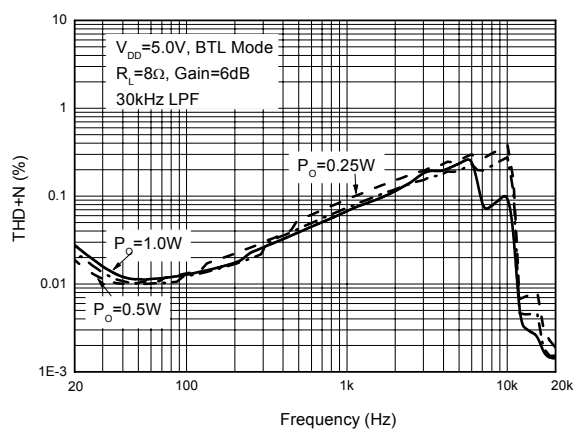
Figure 18. THD+N vs. Frequency
