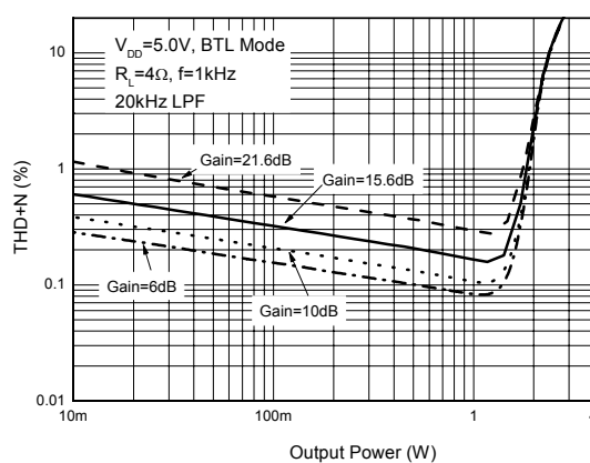
Figure 14. THD+N vs. Output Power
