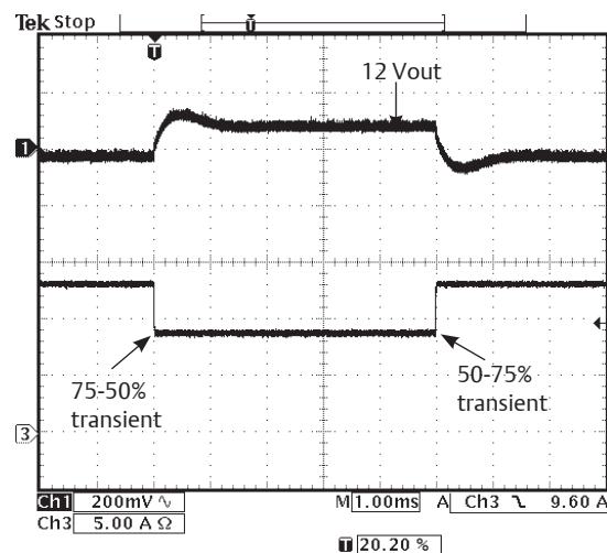
Figure 12: Typical Transient Response 75-50% and 50-75% Step Load Change (1 A/μs). Channel 1: 12 Vout; Channel 3: Iout (12 Vout). Cout = 6000 mF
