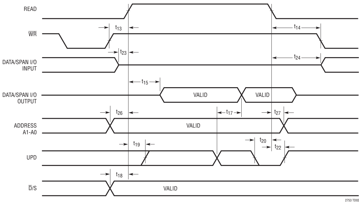
Readback Timing
