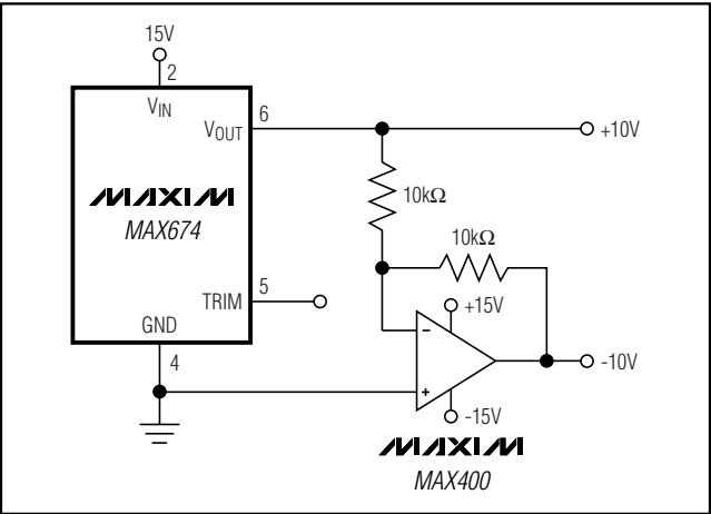
Figure 3. ±10V Reference
