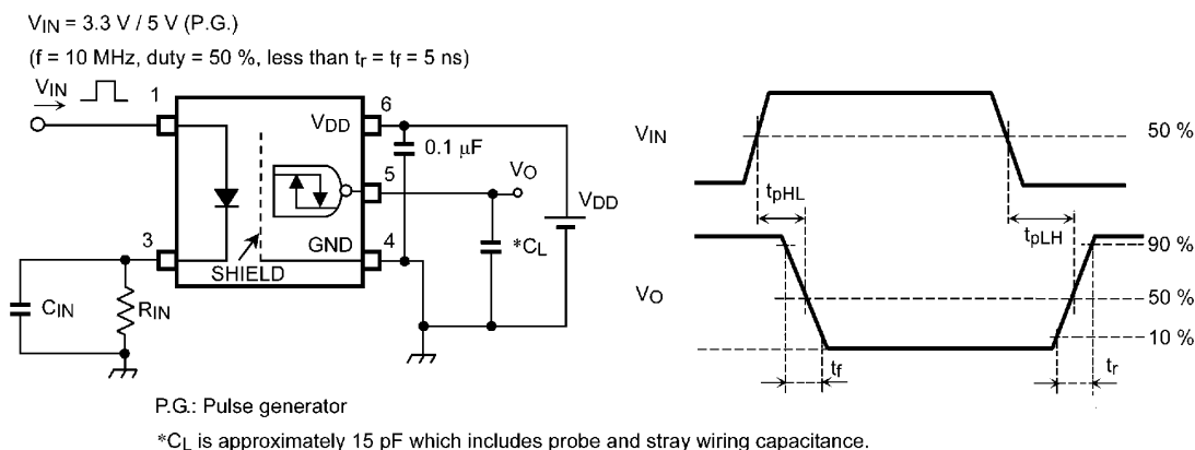
Fig. 12.1.5 Switching Time Test Circuit and Waveform
