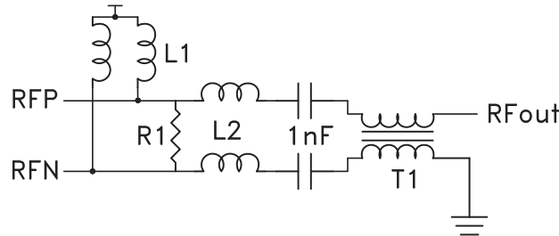
Figure 12. Simple output matching network
