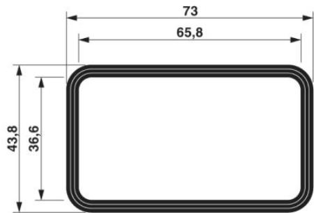
Dimensioned drawing
