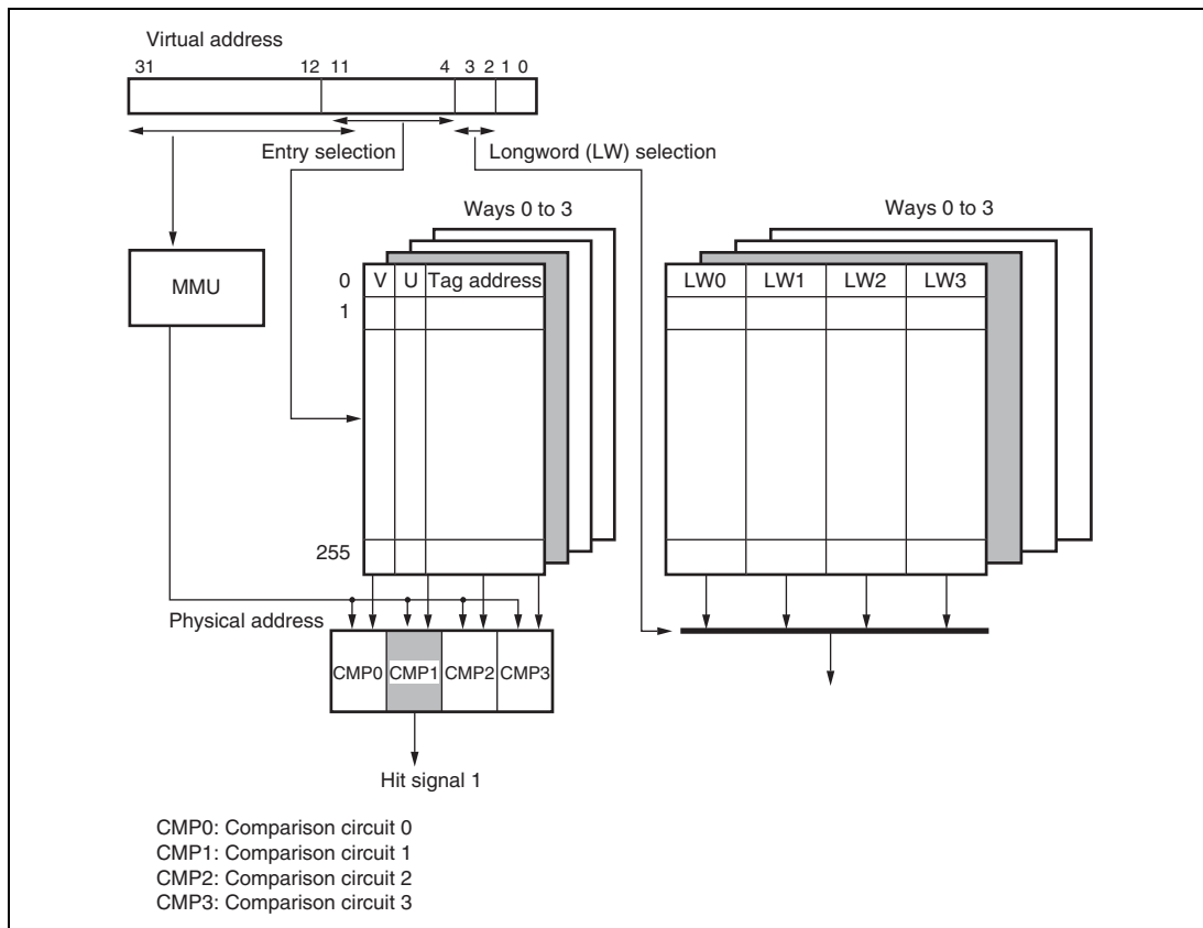
Figure 5.2 Cache Search Scheme
