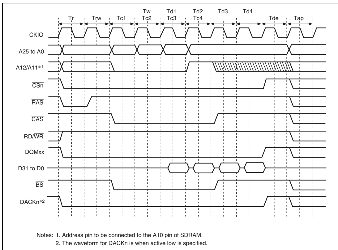
Figure 9.15 Burst Read Wait Specification Timing (Auto-Precharge)
