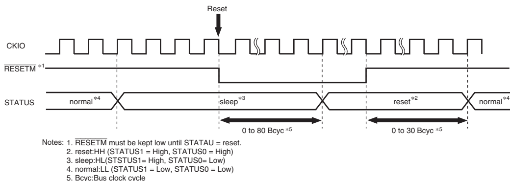
Figure 13.9 STATUS Output When Sleep Mode is Canceled by a Manual Reset
