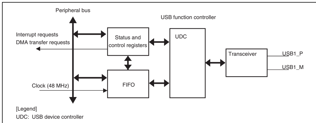
Figure 25.1 Block Diagram of USBF
