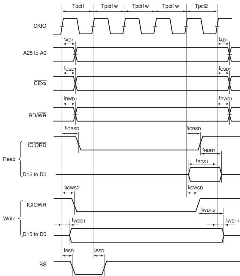
Figure 38.41 PCMCIA I/O Card Interface Bus Timing
