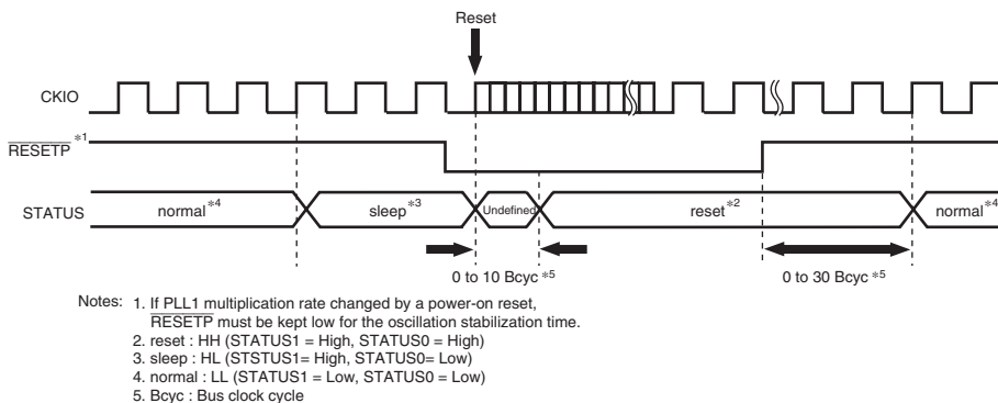
Figure 13.8 STATUS Output When Sleep Mode is Canceled by a Power-on Reset
