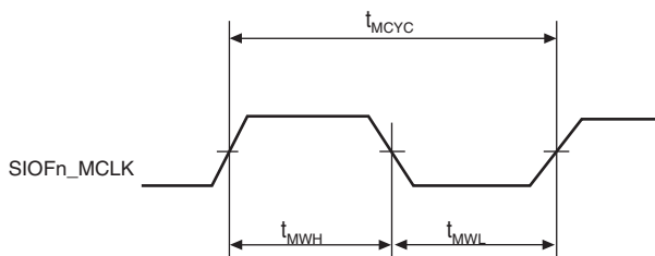
Figure 38.53 SIOF_MCLK Input Timing
