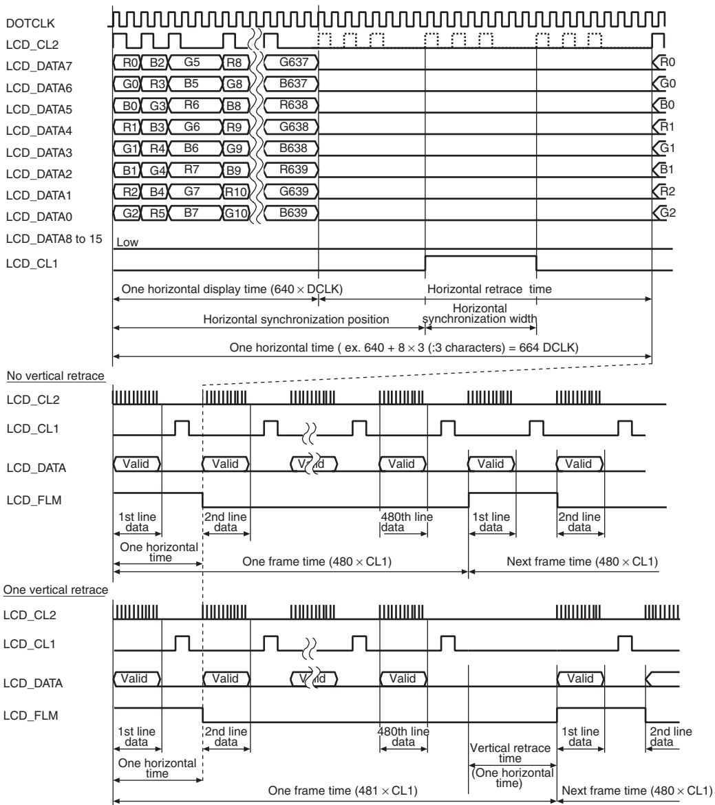
Figure 26.22 Clock and LCD Data Signal Example (8-Bit Interface Color 640 × 480)
