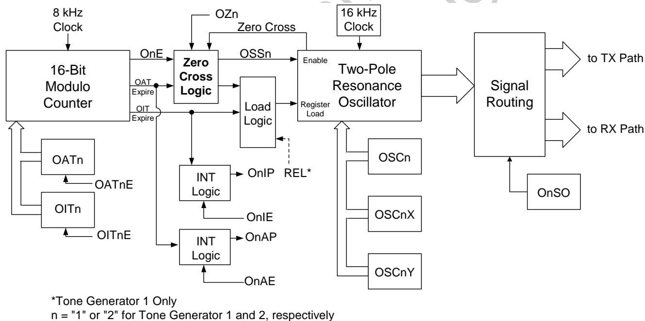
Figure 20. Simplified Tone Generator Diagram
