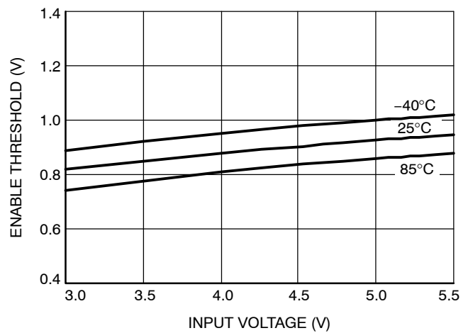
Figure 14. EN/PWM Threshold vs. VIN
