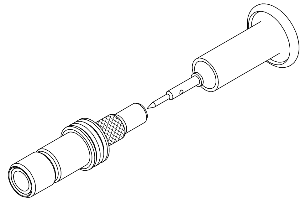
ISOMETRIC VIEW
