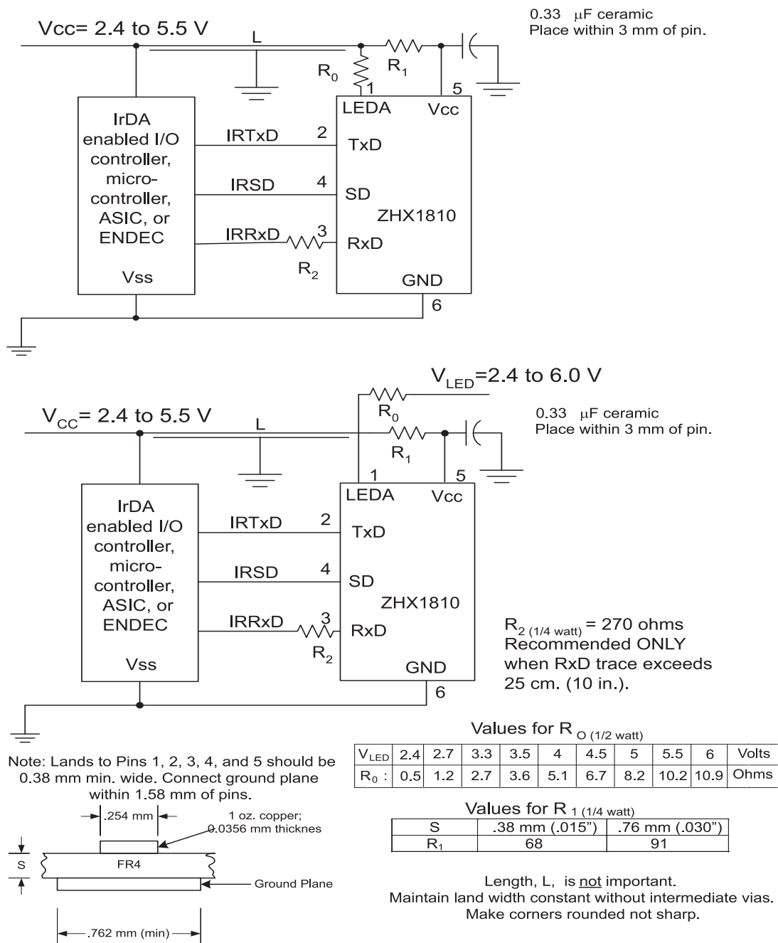
Figure 2. Application Block Diagrams
