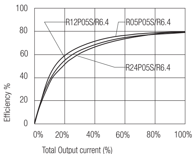
Efficiency / Load
