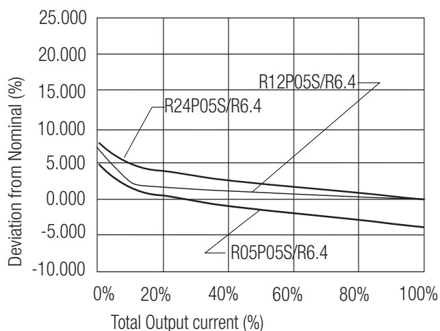
Deviation / Load
