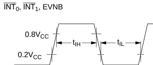
Figure 85 Interrupt Timing
