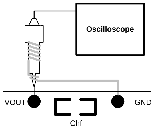
Figure 3. Voltage Ripple Measurements
