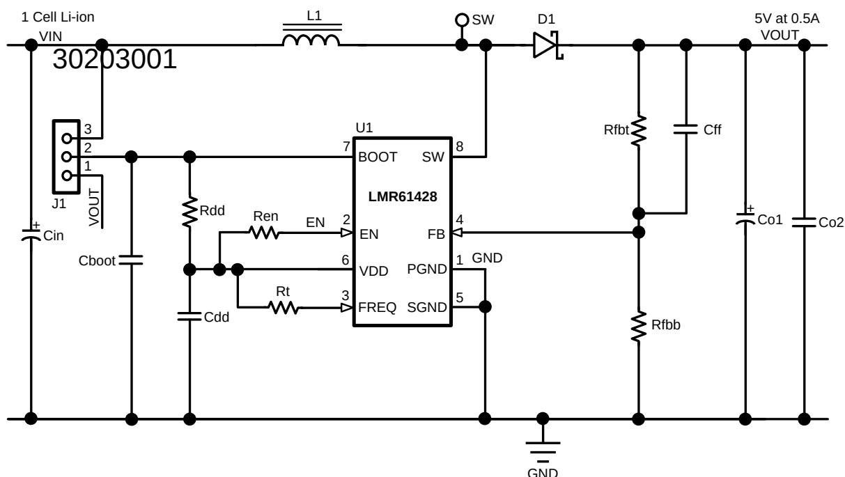
Figure 1. LMR61428 Evaluation Module Schematic
