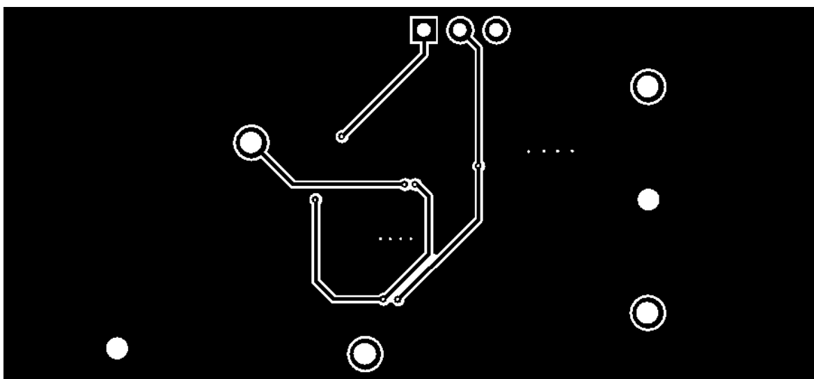
Figure 10. Internal Layer 2
