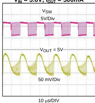
Switching Node and Output Voltage Waveforms V_{IN} = 3.6V, I_{OUT} = 500mA
