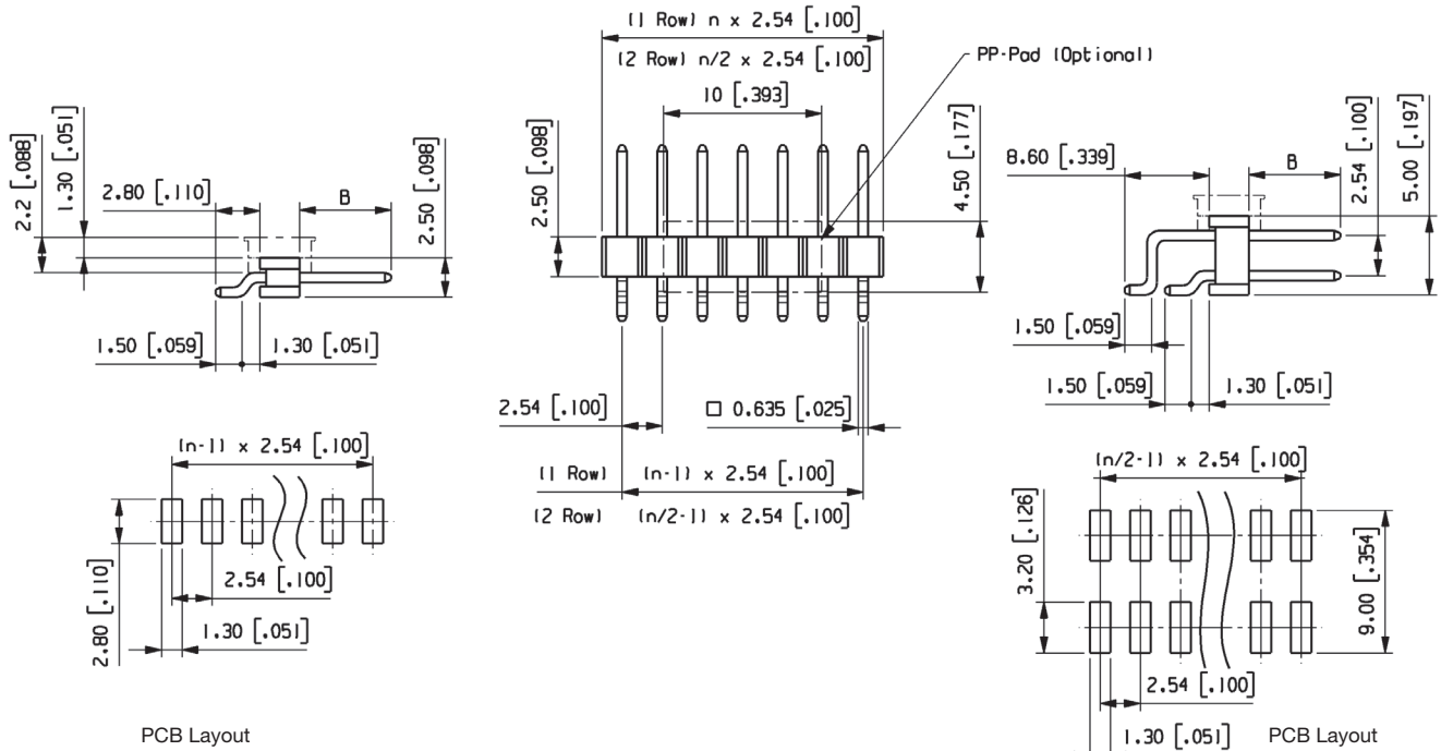
PCB Layout
