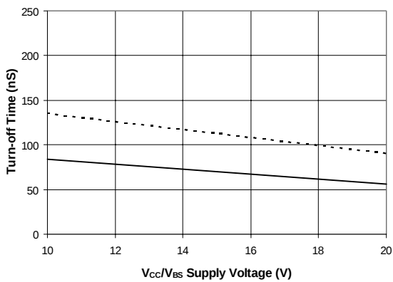
Figure 8B. Turn-off Time vs. Vcc/Vbs Voltage
