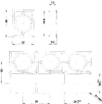
panel cutout
