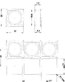
panel cutout
