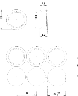
panel cutout
